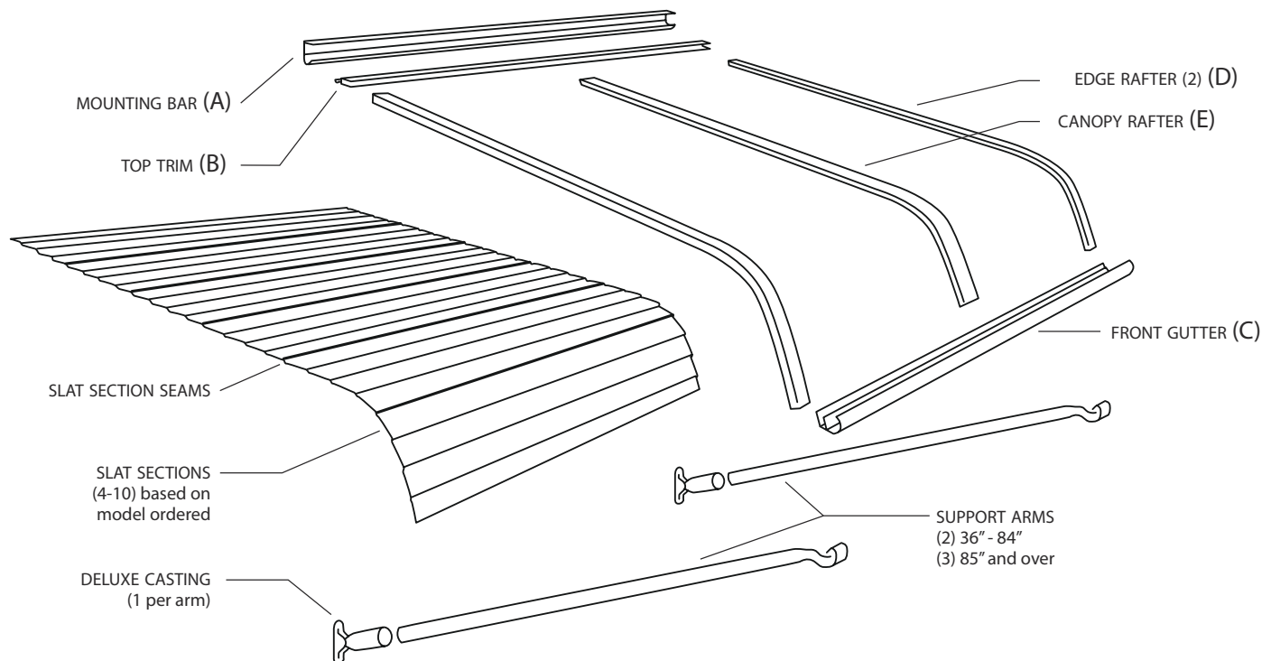
Door Canopy with Support Arms
